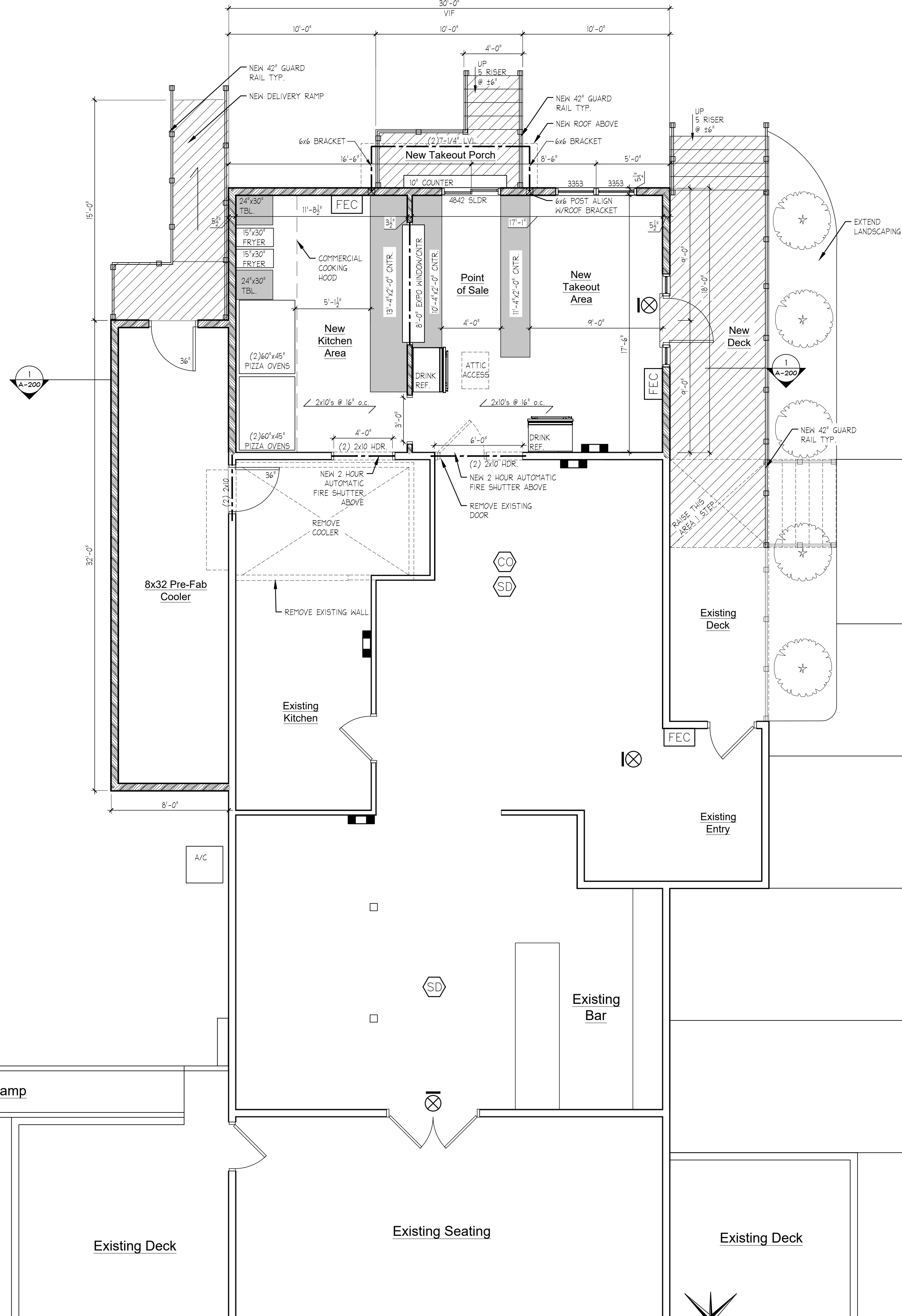
2 First Floor Plan 1/4"=1'-0"
