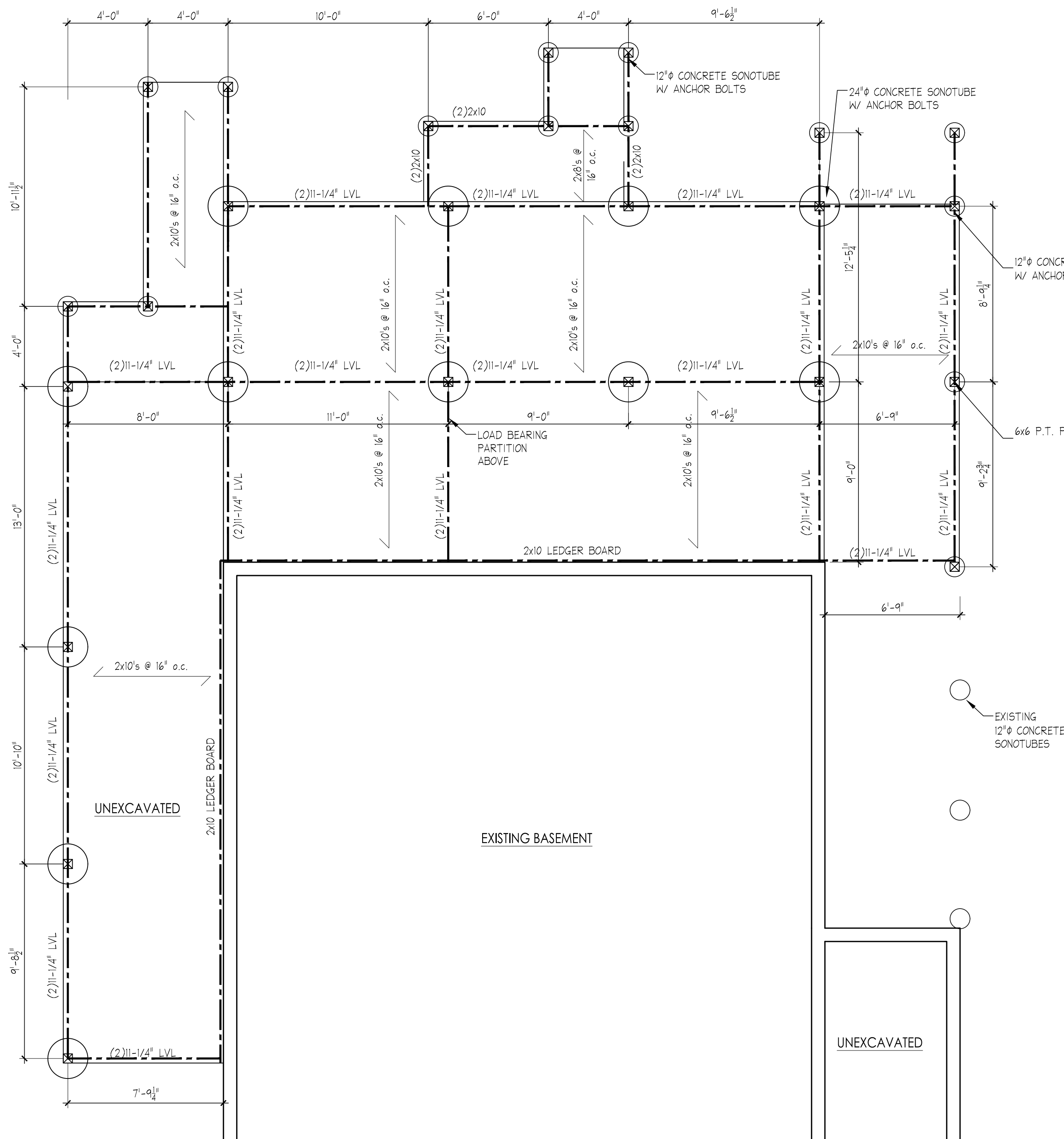
1 Foundation Plan 1/4"=1'-0"
